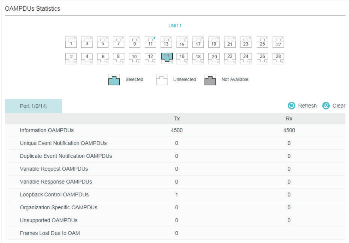
Figure 3-1 OAMPDUs Statistics
