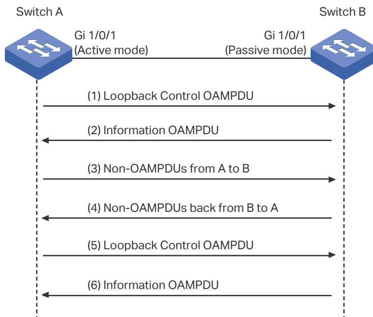
Figure 1-2 Remote Loopback
