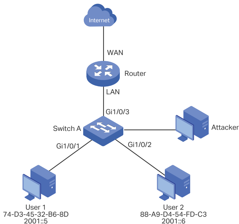
Figure 5-1 Network Topology
