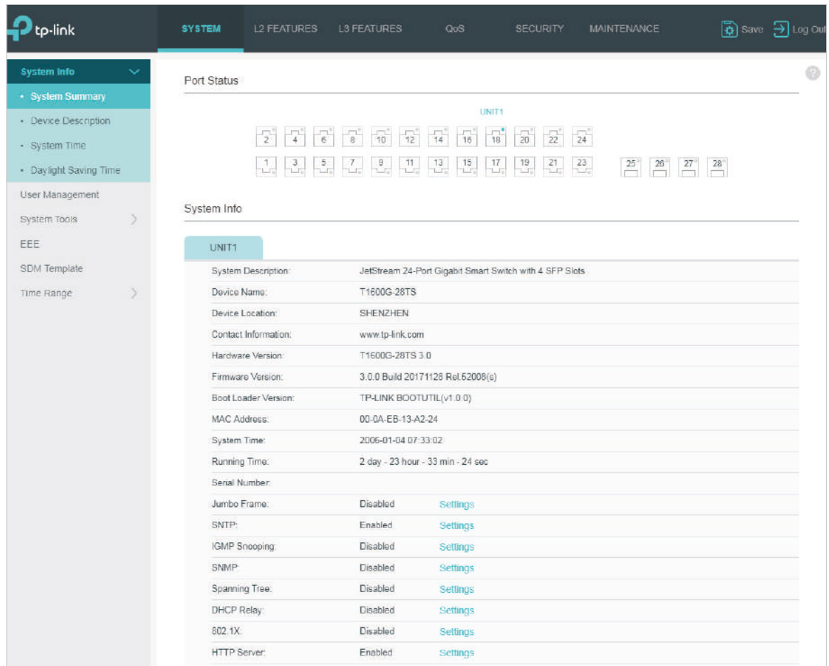
Figure 2-3 Web Interface
