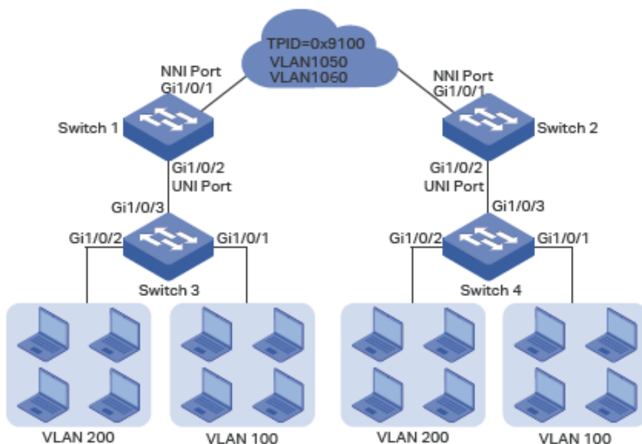
Figure 4-10 Network Topology
