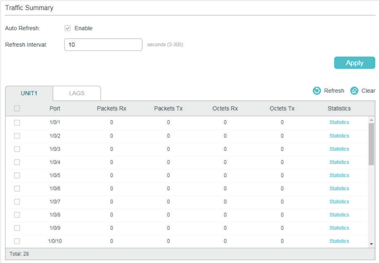
Figure 1-1 Traffic Summary
