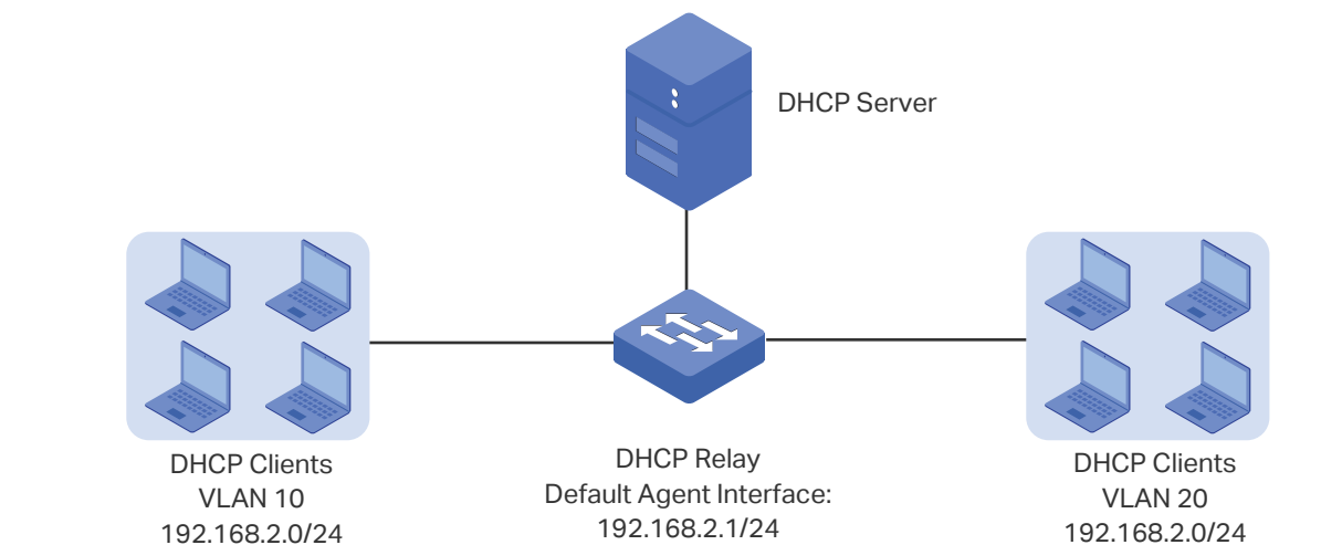
Figure 1-3 Application Scenario of DHCP VLAN Relay
