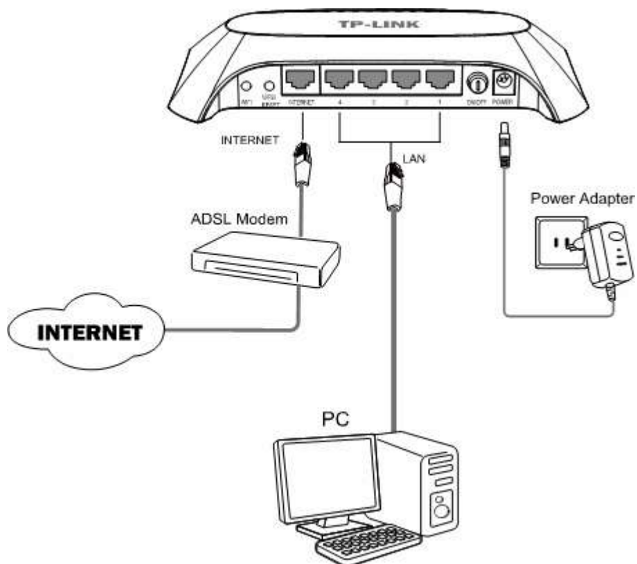
Figure 2-1 Hardware Installation
