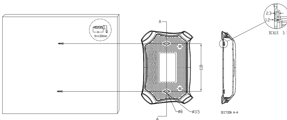
Figure 2-2 Wall-mount Install
